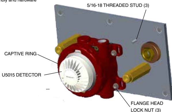
Figure 7—U5015 Smoke Detector mounted on Q5016 plate assembly
