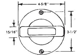
Surface Mounting Unit for Exposed Wiring
